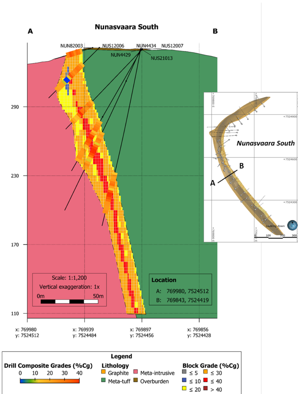
Figure 4 Cross Section through the Nunasvaara South Graphite Deposit
