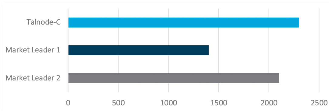
Figure 3 Stelvio Test: time (s) for cell voltage to fall below 3.2V, at 14°C. Details of test cycle: discharge 3 seconds at 3C, charge 1 second at 1C, rest for 4 seconds and repeat until voltage or thermal limit.
