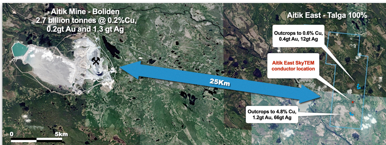
Figure 4 Talga's Aitik East project and SkyTEM anomaly location. See Fig 5 for survey location details.
